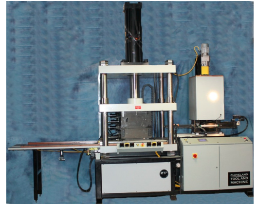
CTM-CI-100 100 ton ceramic injector with shuttle table and outboard pattern ejection.
